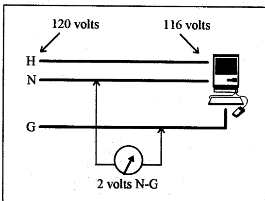
Figure 2 - Voltage Drop at Long Branch Receptacle
