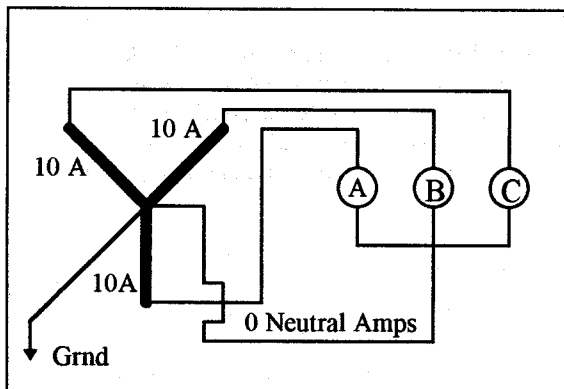
Figure 1 - Shared Neutral in 3 Phase Wye Distribution
