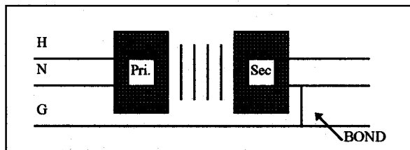
Figure 5 - Output Neutral to Ground Bond
